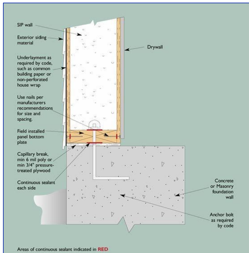
Cross section detail of a typical SIP and the wall to foundation connection. (Source: www.sips.org)
